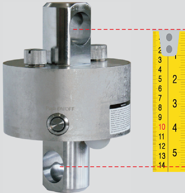
ANYLOAD wireless 10t crane scale
