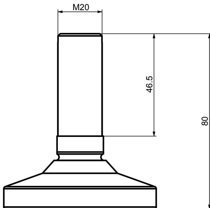
SBF13K-1 Dimensions in mm.
