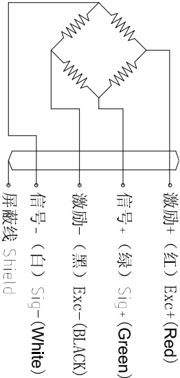
接线图Wiring Schematic Diagram
